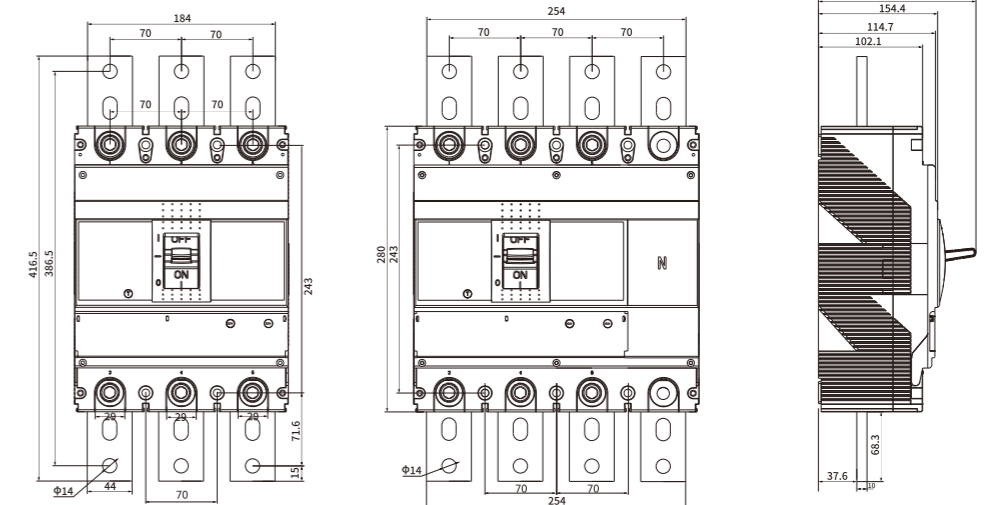
VGM6/6s/6sm/6E-800A 3 POLES & 4 POLES
