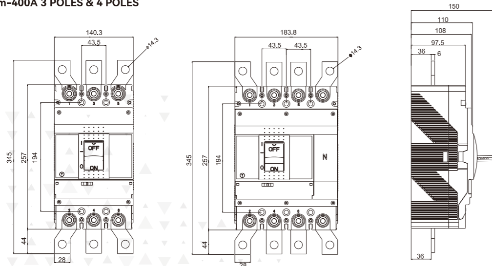
VGM6/6s/6sm-400A 3 POLES & 4 POLES
