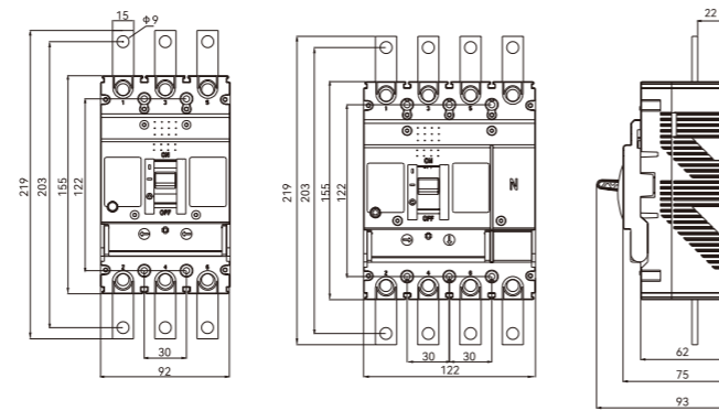
VGM6/6s/6sm-160A 3 POLES & 4 POLES
