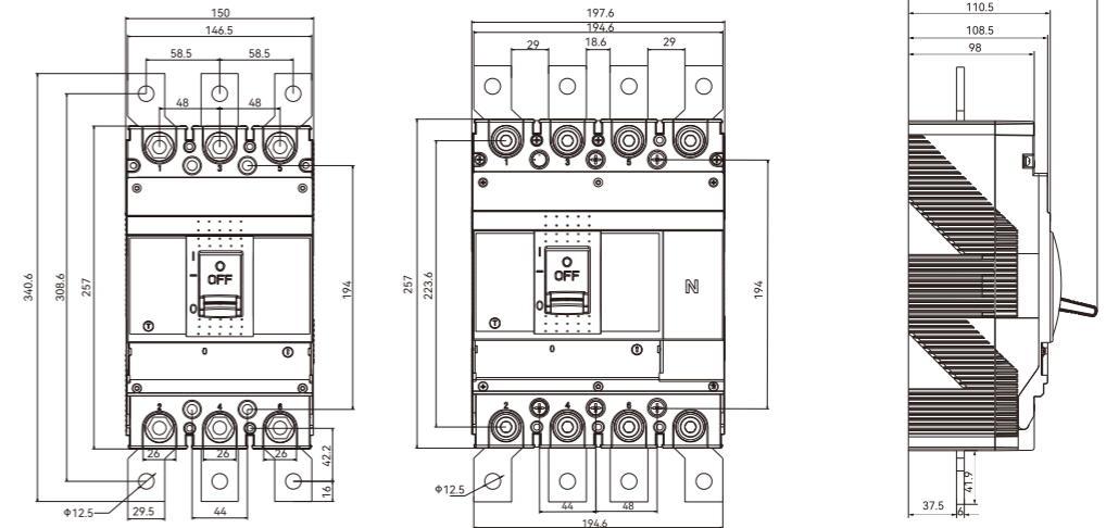
VGM6/6s/6sm/6E-630A 3 POLES & 4 POLES
