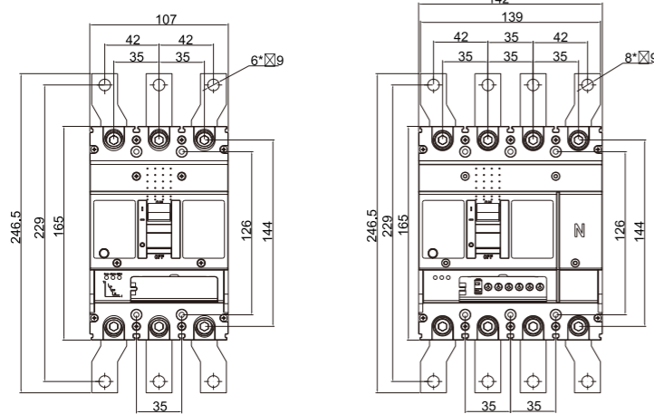
VGM6/6s/6sm/6E-250A 3 POLES & 4 POLES
