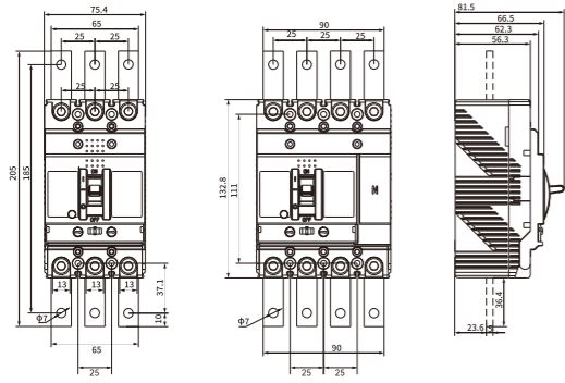
VGM6/6s-125A 3 POLES & 4 POLES VGM6
