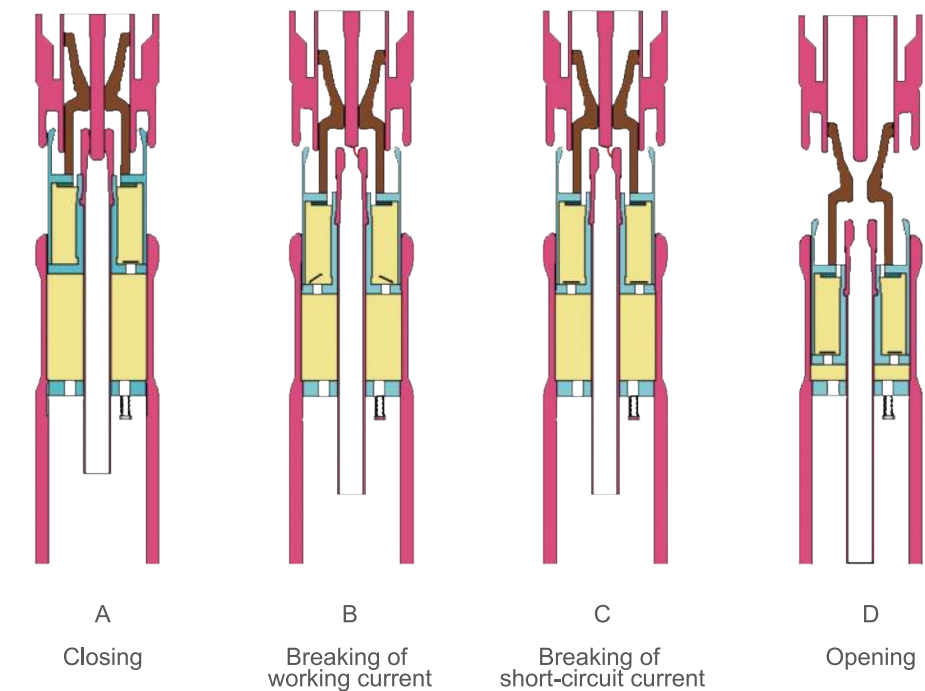
Schematic Diagram of Arc Extinguishing Principle of Self-energized Arc Extinguishing Chamber
