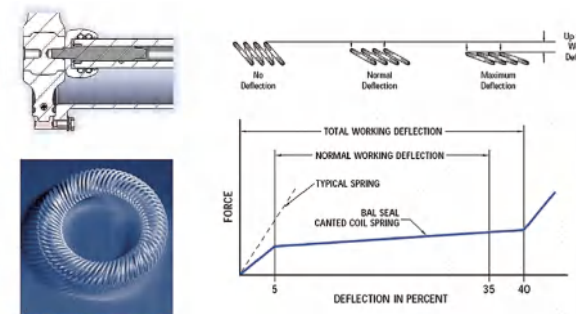
Mechanical Characteristics of Spring
