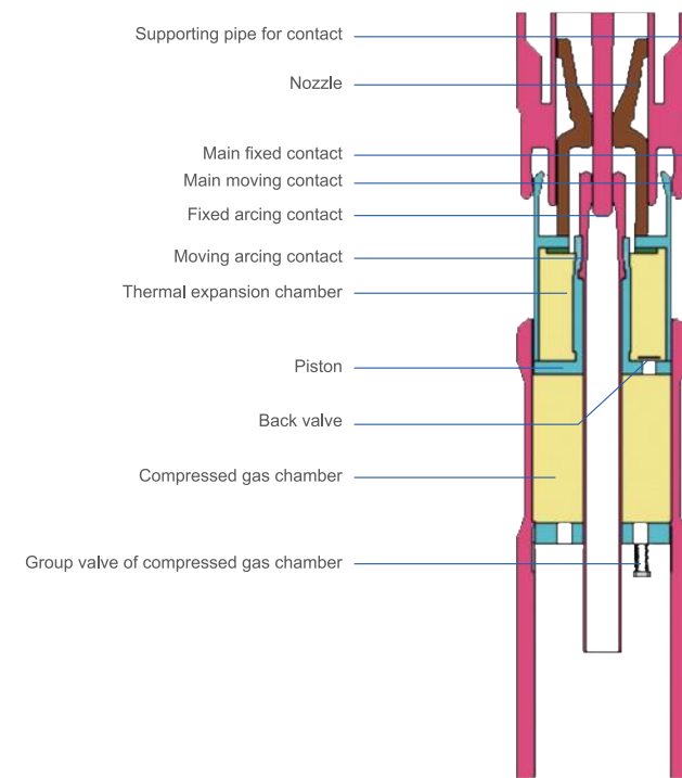
Schematic Diagram of Self-energized Arc Extinguishing Chamber
