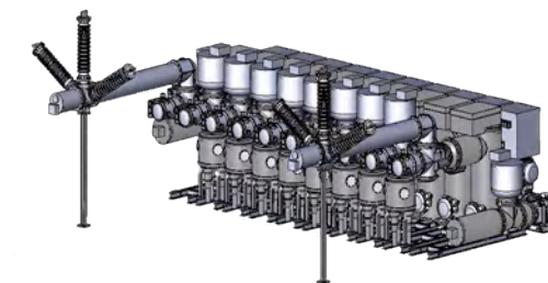
Overhead Incoming for Double Bus
